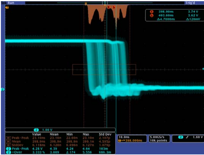
Analyze – Waveform histogram of a falling edge showing the distribution of edge position (jitter) over time. Included are numeric measurements made on the waveform histogram data. A comprehensive set of integrated analysis tools speeds verification of your design's performance.
